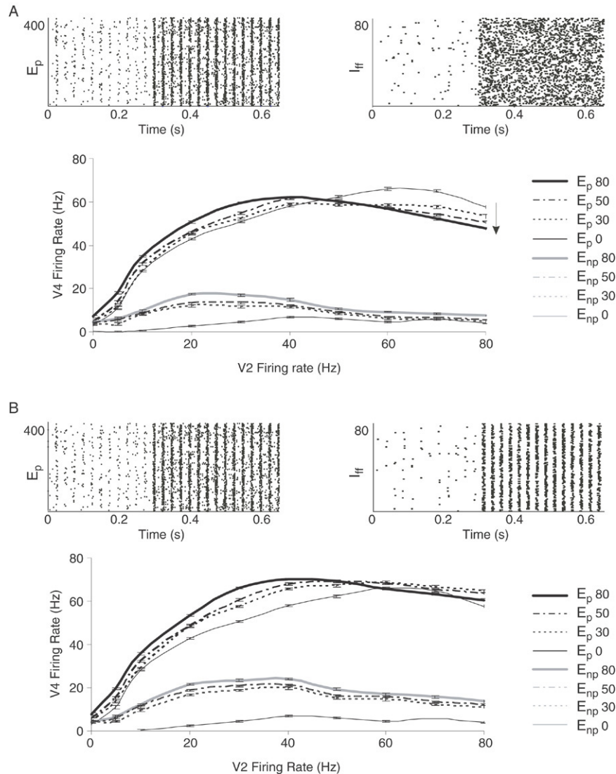
Fig. 7. Modulation of the firing rate of the modeled V4 neuron by combinations of correlations in the excitatory and inhibitory input synapses. (A) Top: Rastergrams depicting correlated input spike activity from the preferred ( E_p ) synaptic population (left) and the non-correlated input spikes from the inhibitory pool ( I_{ff} , right). In this examples 80% of excitatory synapses were correlated at a 40 Hz oscillation rhythm. Simulated activity of the V4 neuron to such input is shown below the rastergrams. The thin black line depicts the baseline response to the preferred stimulus without any correlation in the synaptic inputs (P 0). Effect of 30%, 50% and 80% preferred excitatory input correlations are represented by the dotted black line (P 30), dot dashed black line (P 50) and thick black line (P 80) respectively. The thin gray line is the baseline response to the non-preferred input without any correlations in the excitatory input (NP 0). Effects of increasing correlation percent to 30%, 50% and 80% are respectively shown by the dotted gray (NP 30), dot dashed gray (NP 50) and thick gray (NP 80) lines respectively. Response increase is seen only at low and intermediate V2 input firing rates. Substantial response suppression occurs at high input firing rates only if the excitatory input is correlated (depicted by arrow). In (B) both excitatory and inhibitory synaptic inputs were correlated at 40 Hz oscillation frequency. Correlations in the inhibitory inputs are 12 ms out of phase with respect to the excitatory inputs. The corresponding V4 neuron response to such input is shown. All inhibitory inputs were correlated while the % correlation in the excitatory input was changed to 30%, 50% and 80%. Line points are same as those used in panel A. The prominent effect of inhibitory input correlations out of phase with the excitatory input is to remove the response suppression at high firing rates seen when only excitatory input is correlated in the preferred condition.
