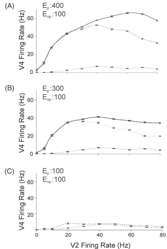
Fig. 4. Response of the modeled V4 neuron to pairs of differentially preferred stimuli. The average firing rate response of the V4 neuron to increasing firing rate of the V2 excitatory input is depicted. Response to the preferred stimulus alone (when only V2 E_p is active) is in solid black, and to the non-preferred stimulus alone (when only V2 E_{np} is active) is in light gray. Response to both populations being active at equivalent firing rates is represented by the dashed black line. In all cases E_{np} is modeled with 100 excitatory synapses. In (A), (B) and (C) E_p has 400, 300 and 100 active synapses respectively. As E_p and E_{np} become equally preferred, their responses overlap when activated alone, and hence the solid black line is not visible (C).
